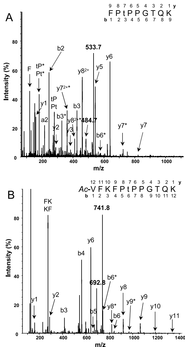
Fig. 2. Sequencing of two phosphopeptides released by trypsin from the isolated thylakoid membranes. Fragmentation spectra of doubly protonated peptide ions with m/z 533.7 (A) and m/z 741.8 (B). The b ion and y ion fragments are indicated in the spectra and in the presented corresponding peptide sequences. The lowercase t designates phosphorylated threonine. Ac- corresponds to the acetylated N-terminal residue in the peptide (B). The ion fragments that contained phosphorylated residue and underwent the neutral loss of H_3PO_4 (mass 98) are marked with asterisks. Some intense internal fragment signals: tP(Pt) and tP*(Pt*) in A and FK(KF) in B, are also marked.
